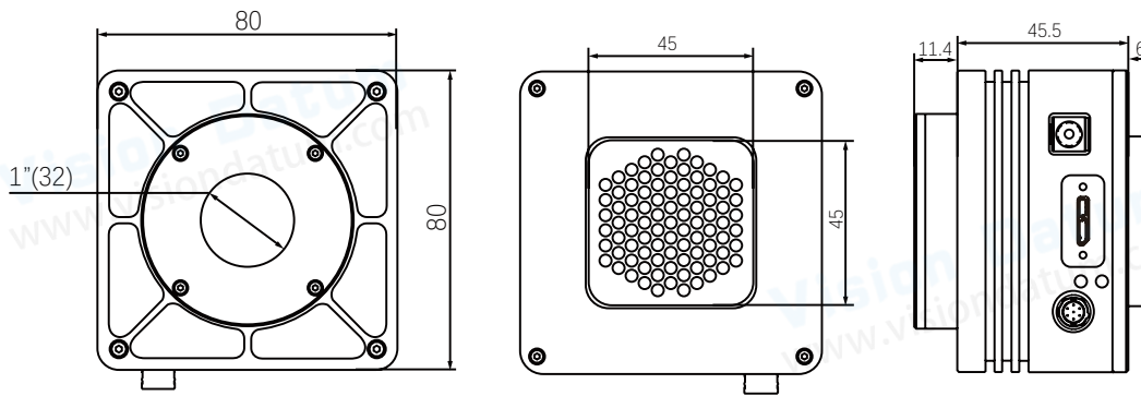
Dimensions A
