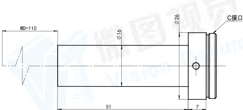
CLW3-ST-0.8X-110
