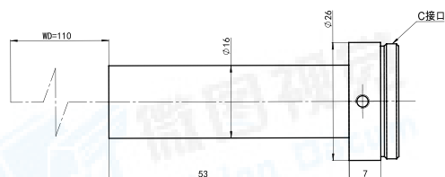
CLW3-ST-1.0X-110
