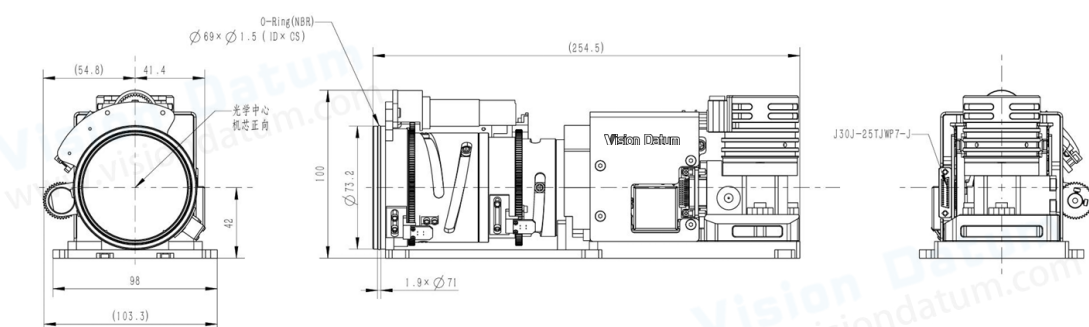
CameraLink 25~75mm Continuous Zoom Lens
