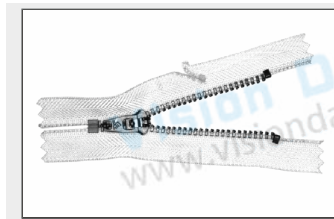
Light: BFCK150100R Imaging of zipper teeth
