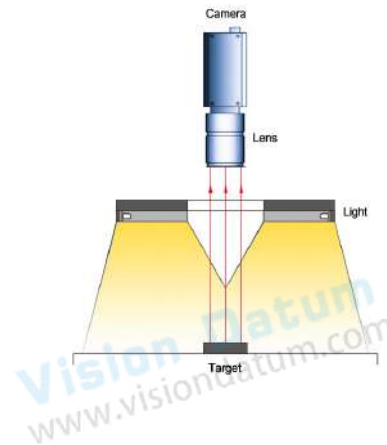
Lights: BFCK250200B Imaging of plastic parts for location.
